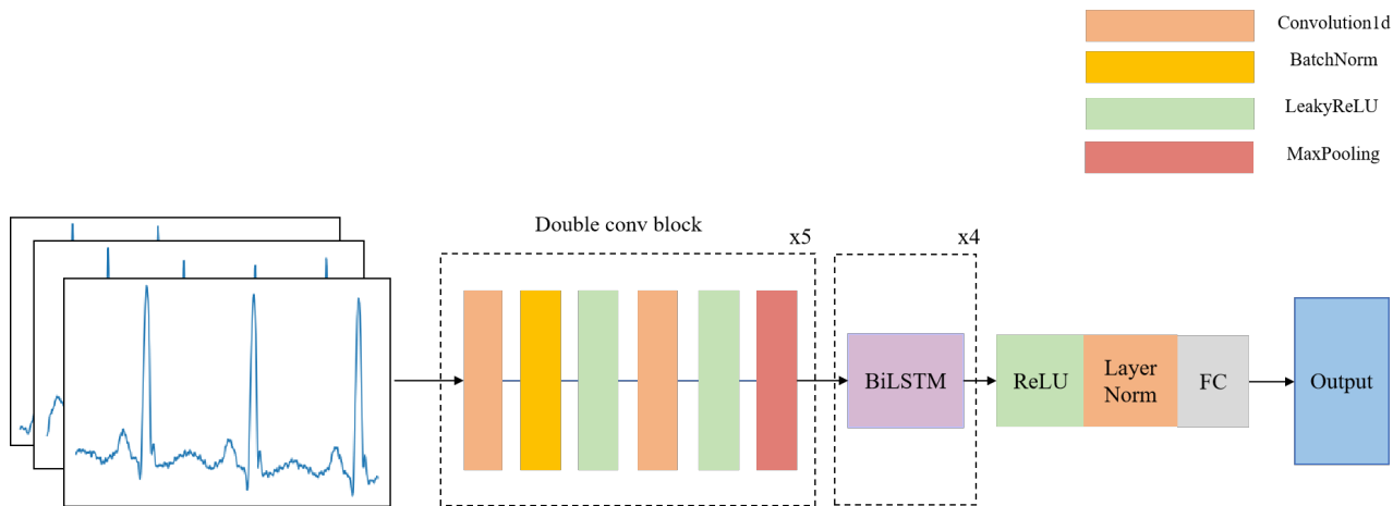
Figure 1. The architecture of MTFNet.
